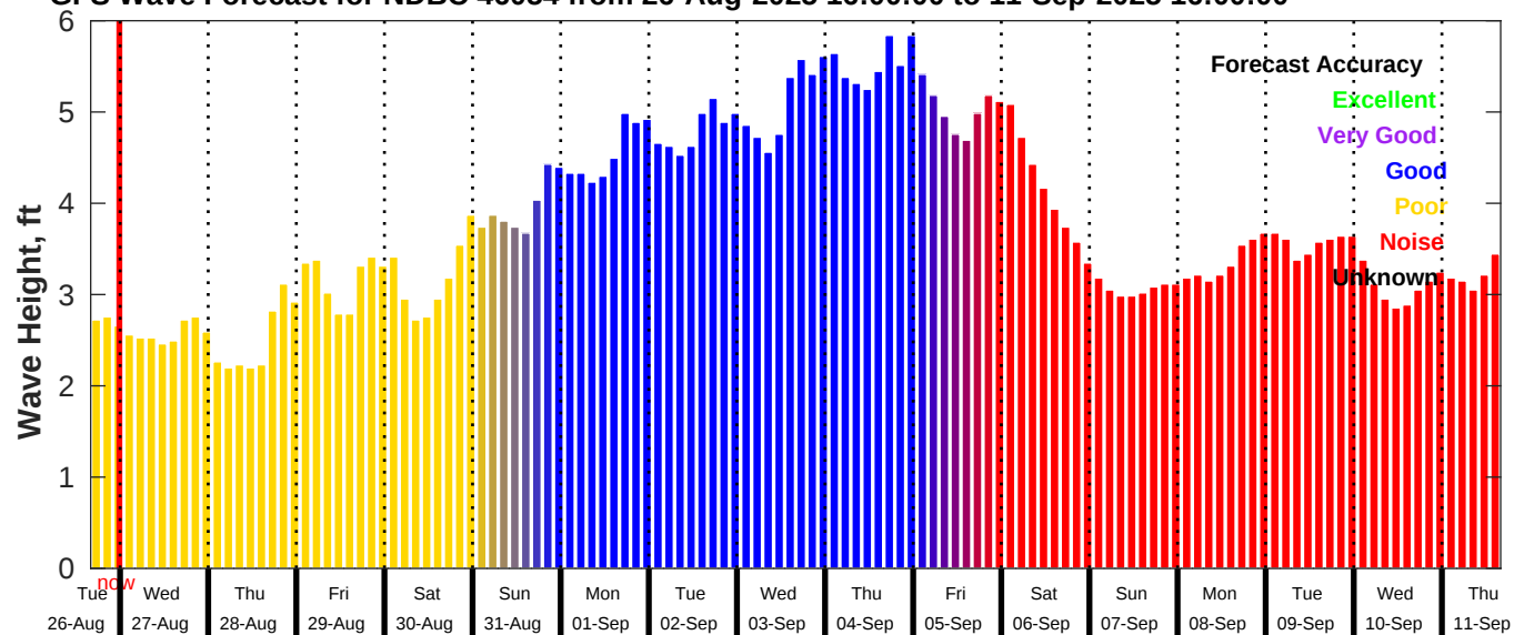
GFS Wave Forecast for NDBC 46054 from 26-Aug-2025 16:00:00 to 11-Sep-2025 16:00:00
