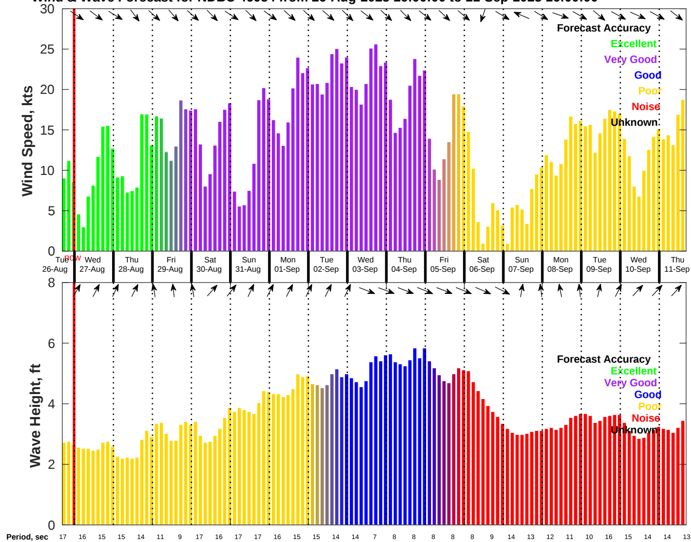
Wind & Wave Forecast for NDBC 46054 from 26-Aug-2025 16:00:00 to 11-Sep-2025 16:00:00
