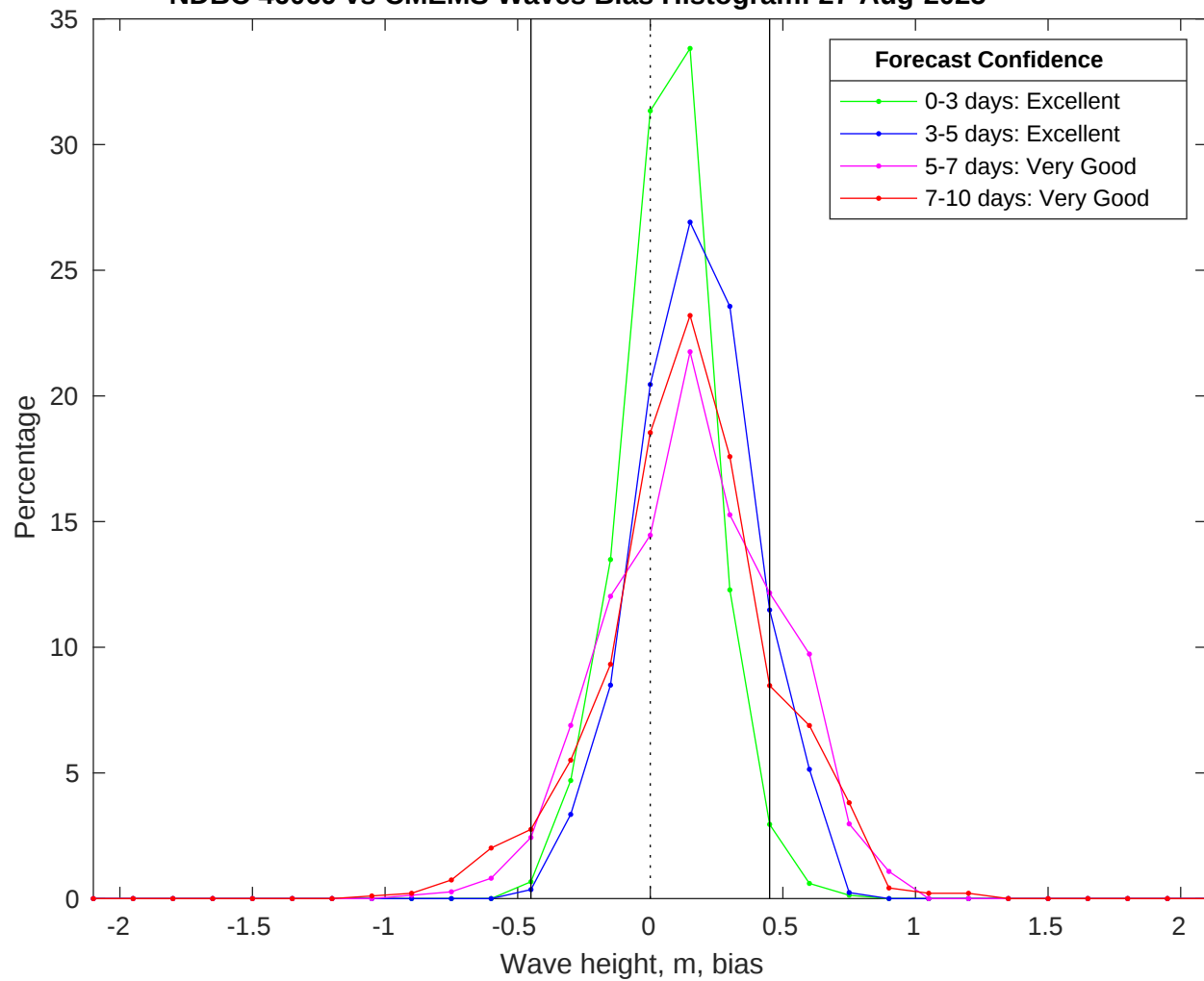
NDBC 46069 vs CMEMS Waves Bias Histogram: 27-Aug-2025
