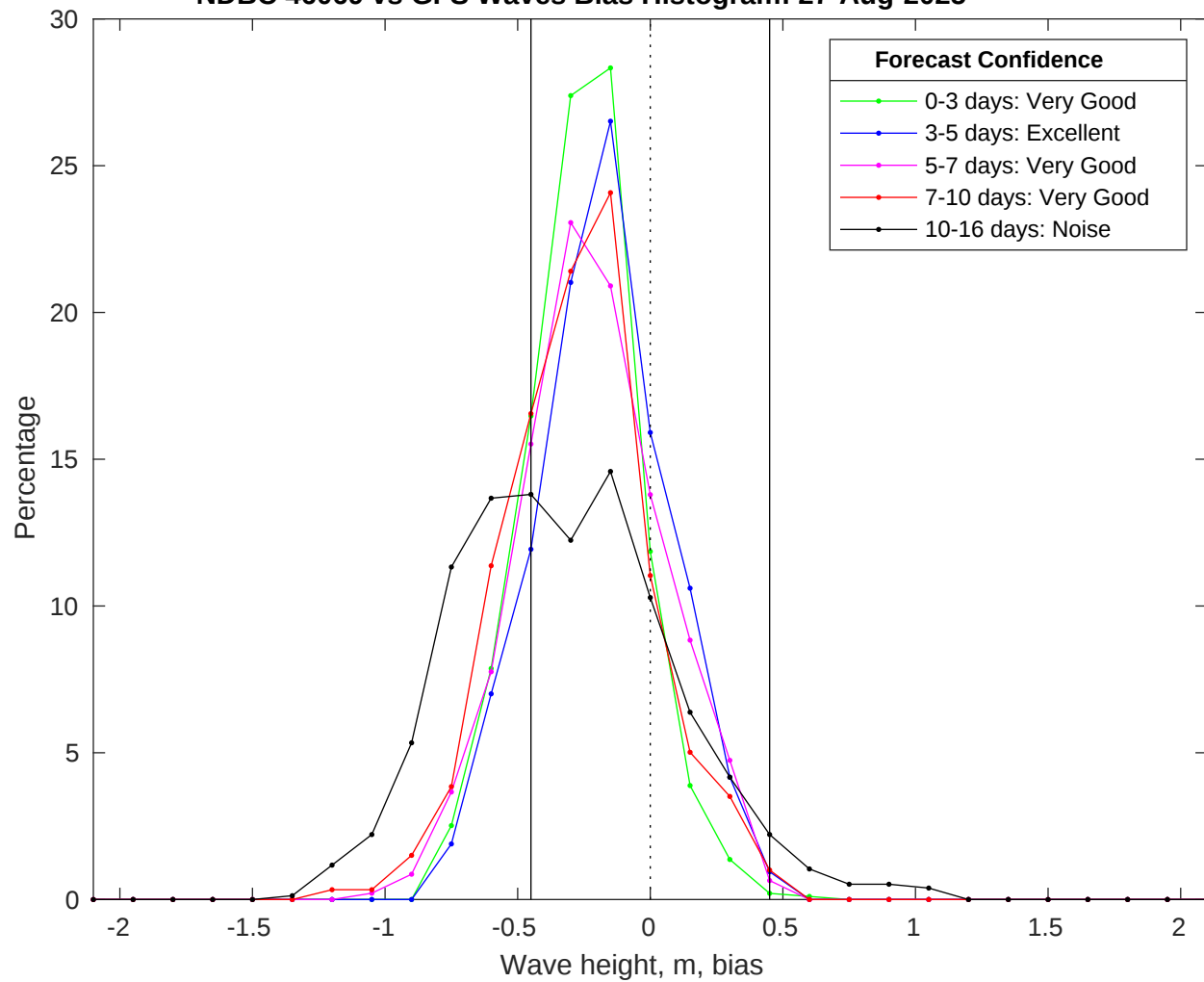
NDBC 46069 vs GFS Waves Bias Histogram: 27-Aug-2025
