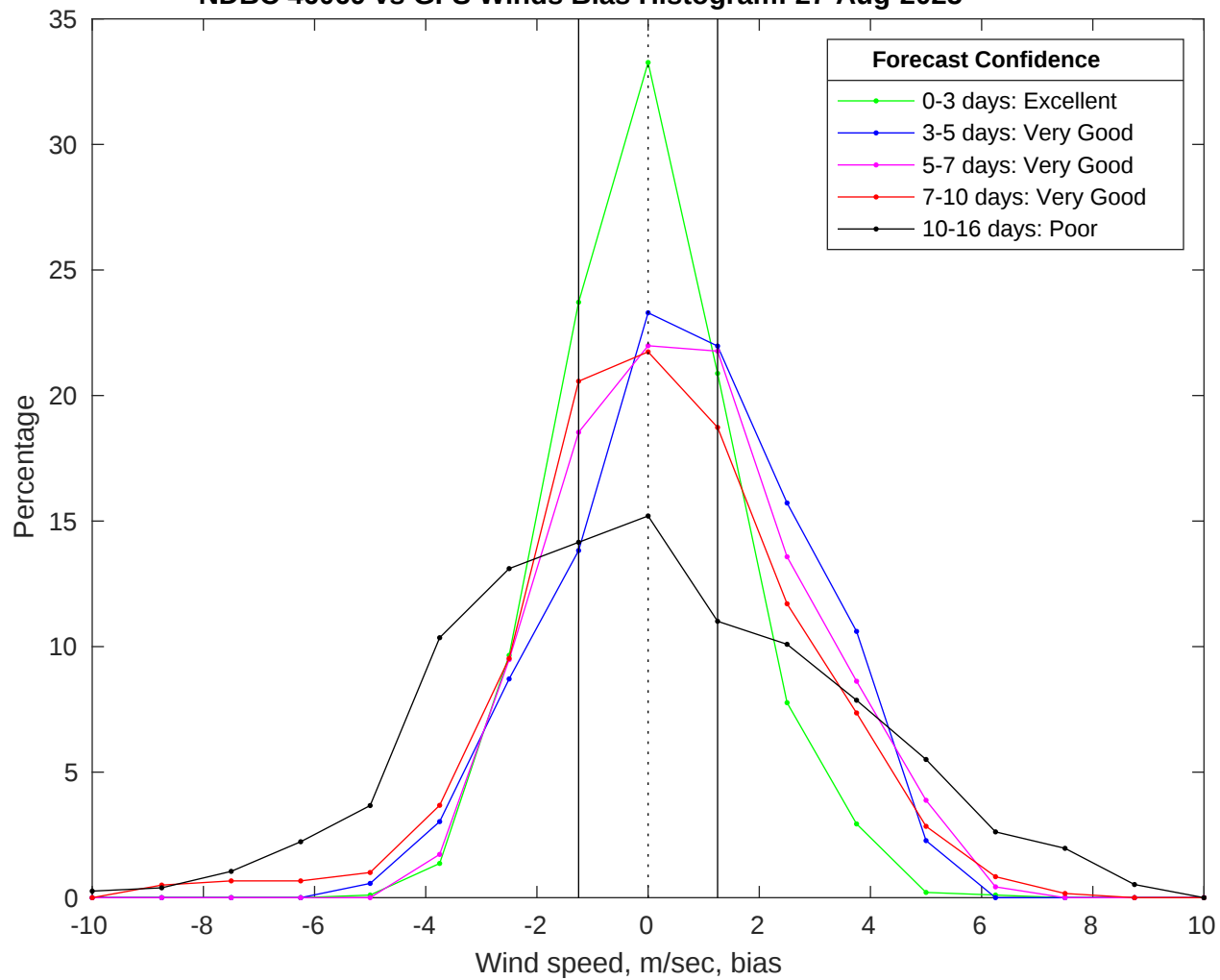
NDBC 46069 vs GFS Winds Bias Histogram: 27-Aug-2025
