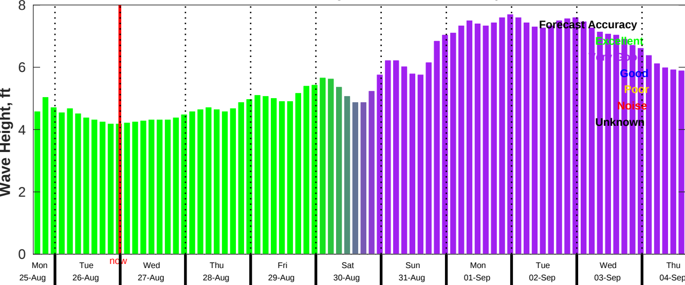
CMEMS Wave Forecast for NDBC 46069 from 25-Aug-2025 16:00:00 to 04-Sep-2025 16:00:00
