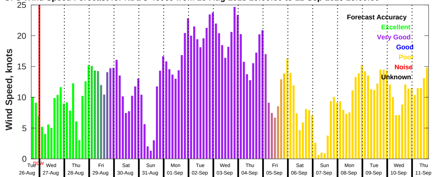
GFS Wind Speed Forecast for NDBC 46069 from 26-Aug-2025 16:00:00 to 11-Sep-2025 16:00:00
