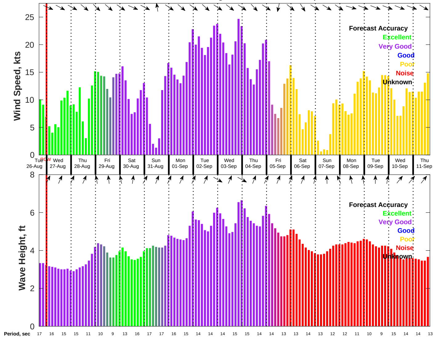
Wind & Wave Forecast for NDBC 46069 from 26-Aug-2025 16:00:00 to 11-Sep-2025 16:00:00
