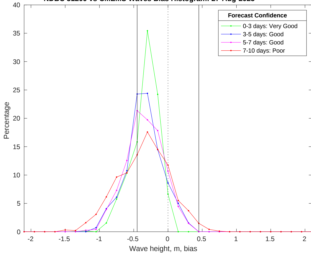
NDBC 51209 vs CMEMS Waves Bias Histogram: 27-Aug-2025
