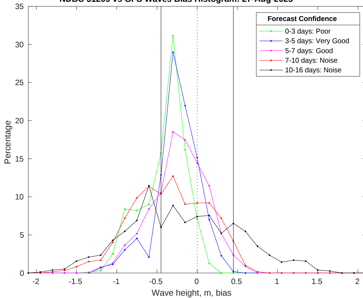
NDBC 51209 vs GFS Waves Bias Histogram: 27-Aug-2025
