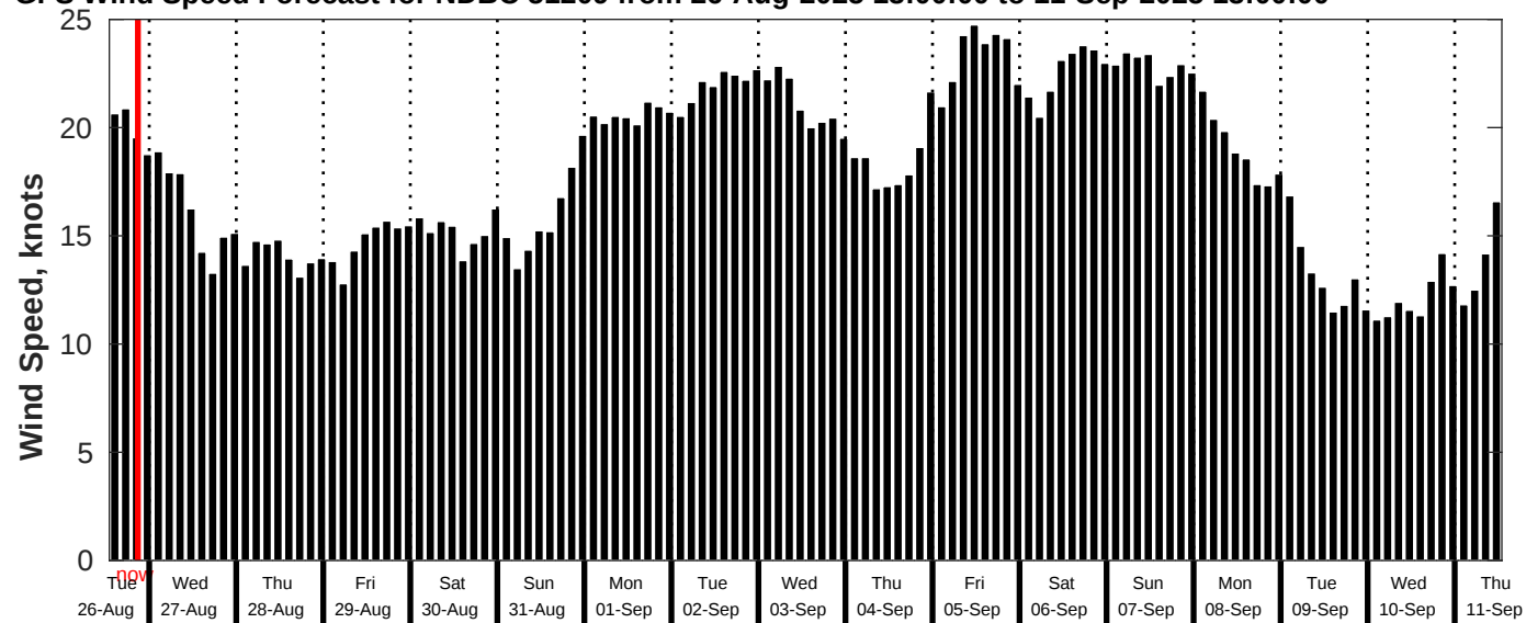
GFS Wind Speed Forecast for NDBC 51209 from 26-Aug-2025 13:00:00 to 11-Sep-2025 13:00:00
