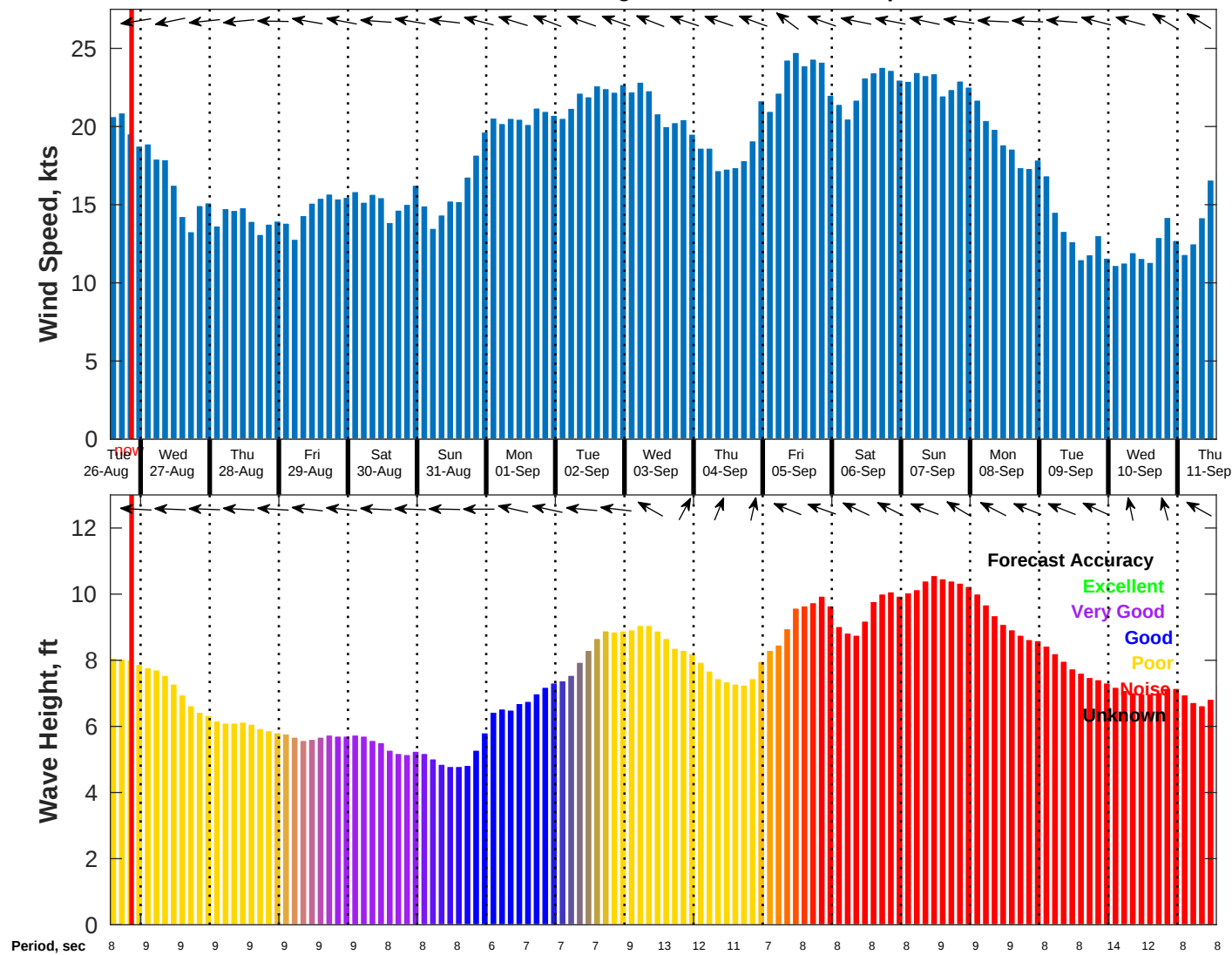
Wind & Wave Forecast for NDBC 51209 from 26-Aug-2025 13:00:00 to 11-Sep-2025 13:00:00
