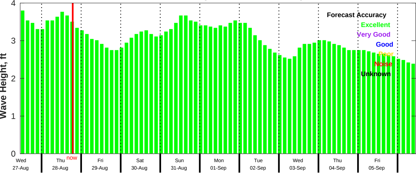
CMEMS Wave Forecast for NDBC 52211 from 26-Aug-2025 11:00:00 to 05-Sep-2025 11:00:00
