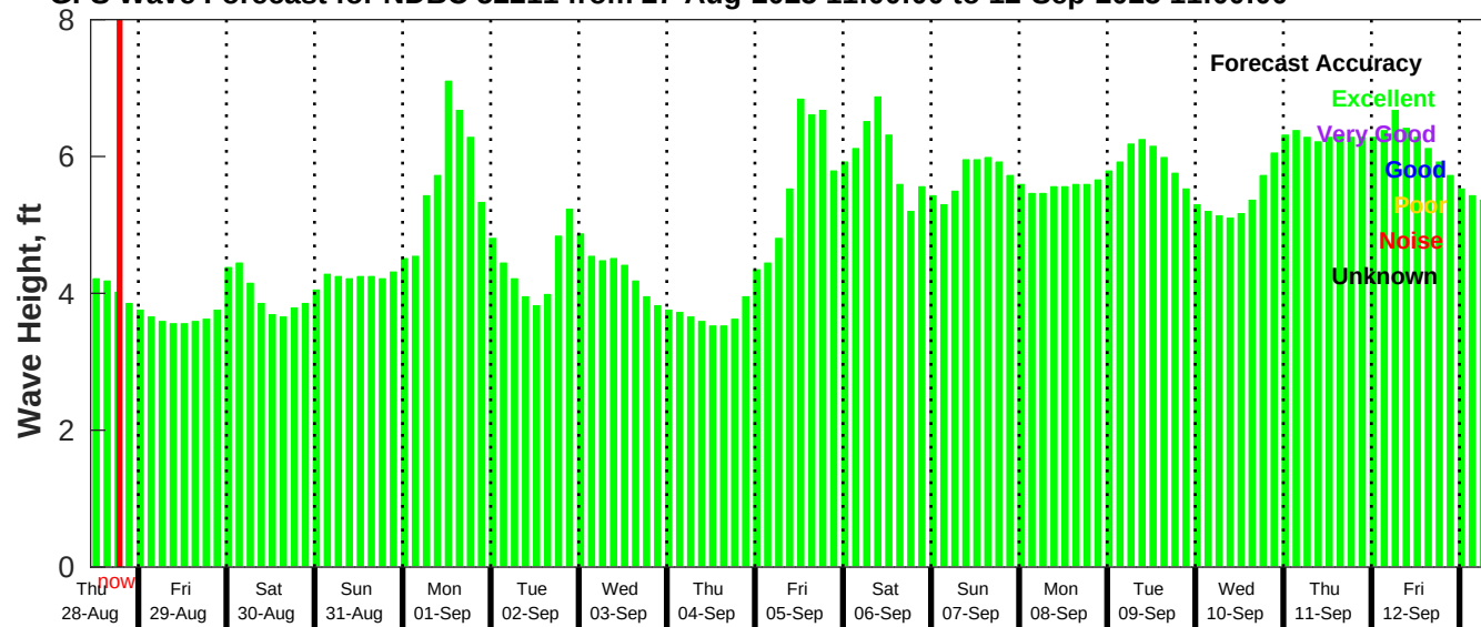
GFS Wave Forecast for NDBC 52211 from 27-Aug-2025 11:00:00 to 12-Sep-2025 11:00:00
