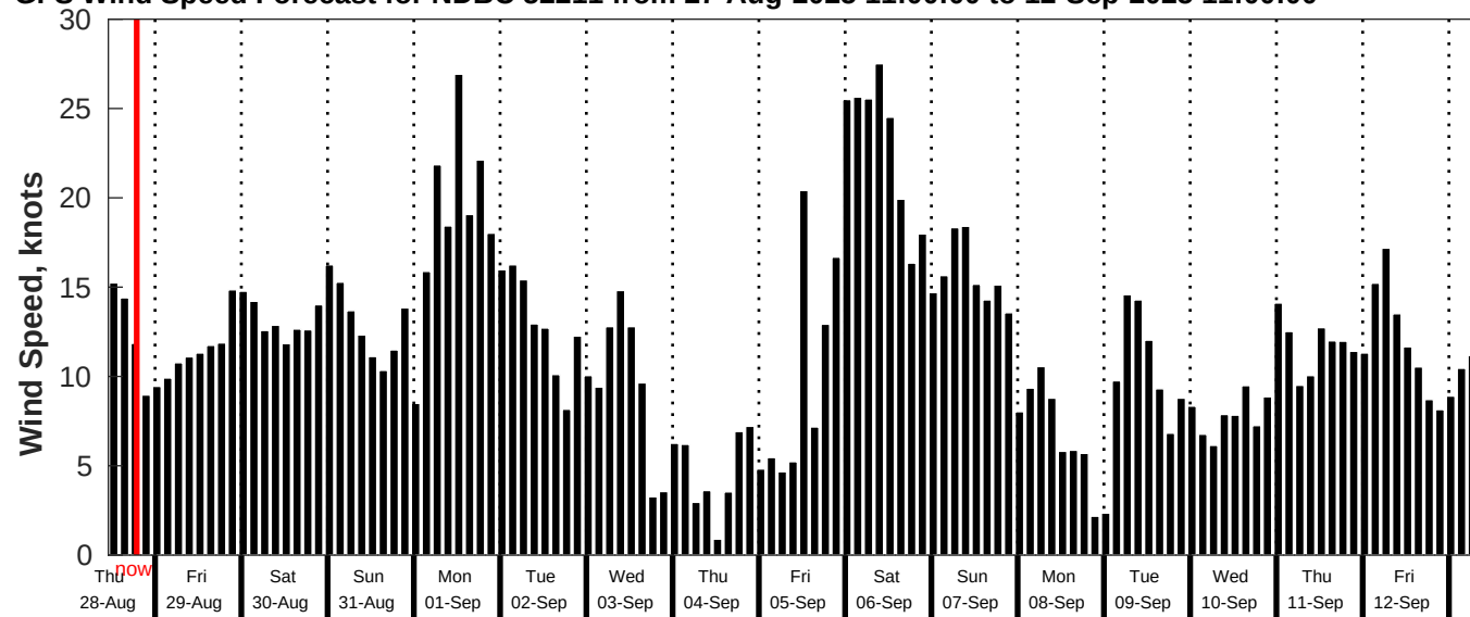
GFS Wind Speed Forecast for NDBC 52211 from 27-Aug-2025 11:00:00 to 12-Sep-2025 11:00:00
