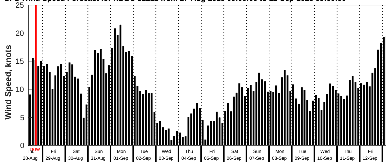
GFS Wind Speed Forecast for NDBC 52212 from 27-Aug-2025 09:00:00 to 12-Sep-2025 09:00:00
