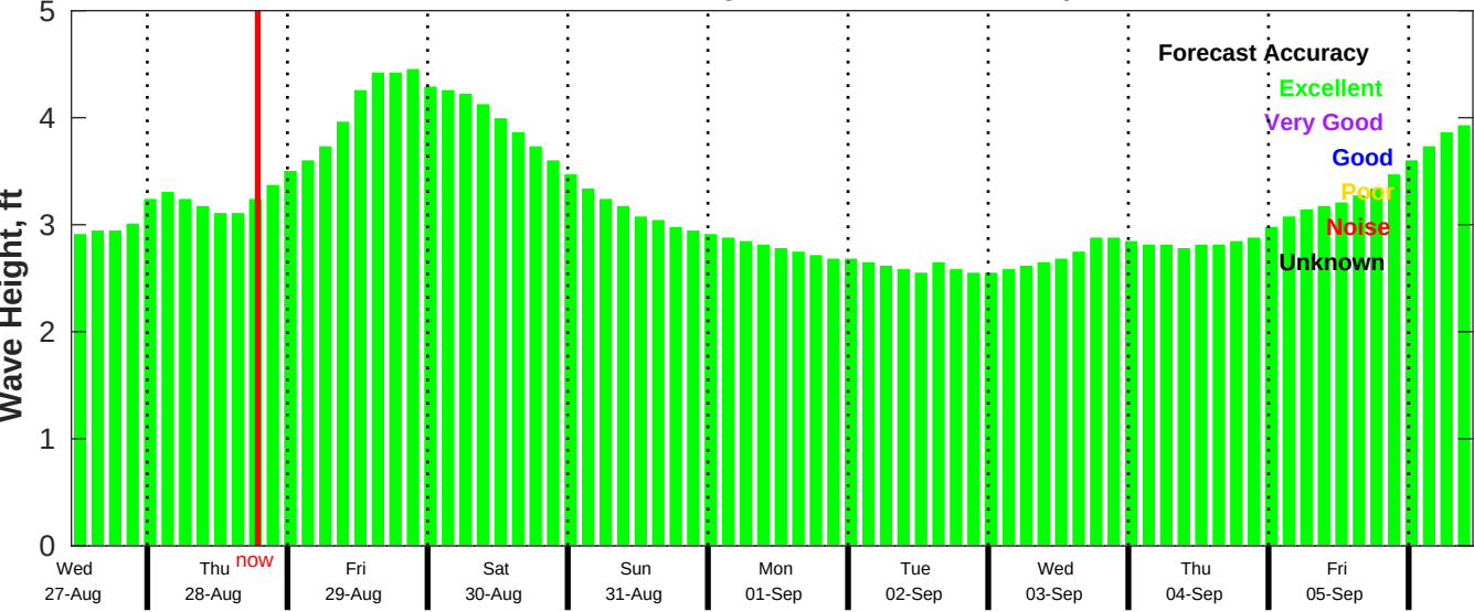
CMEMS Wave Forecast for NDBC 52213 from 26-Aug-2025 11:00:00 to 05-Sep-2025 11:00:00
