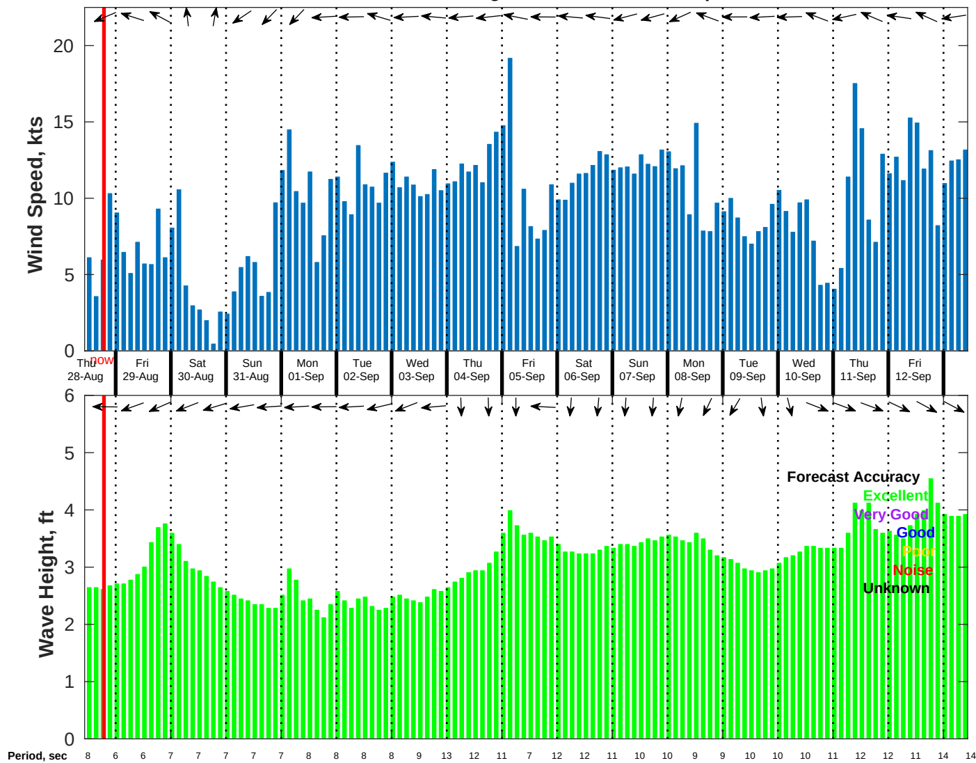
Wind & Wave Forecast for NDBC 52213 from 27-Aug-2025 11:00:00 to 12-Sep-2025 11:00:00
