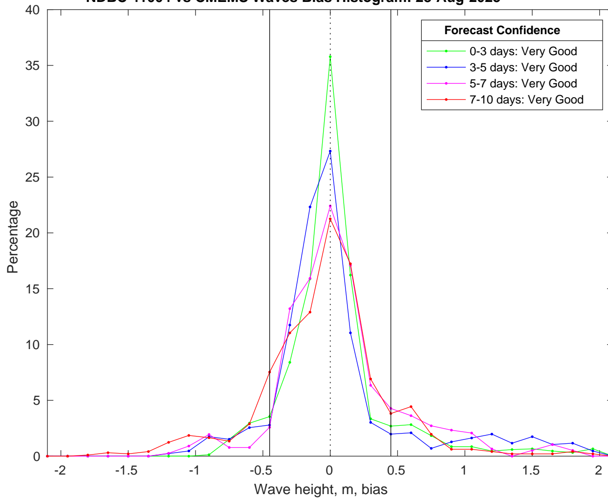
NDBC 41004 vs CMEMS Waves Bias Histogram: 28-Aug-2025
