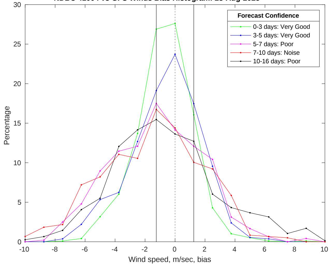
NDBC 41004 vs GFS Winds Bias Histogram: 28-Aug-2025
