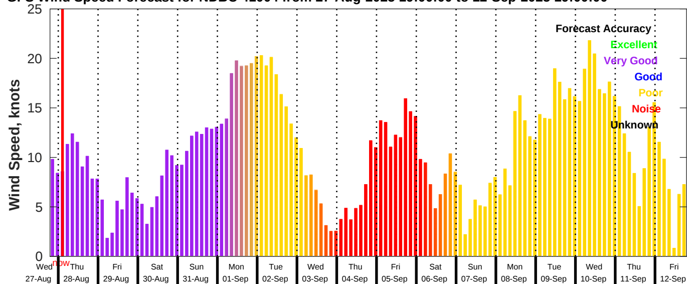
GFS Wind Speed Forecast for NDBC 41004 from 27-Aug-2025 19:00:00 to 12-Sep-2025 19:00:00
