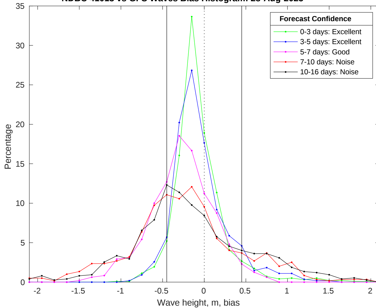
NDBC 41013 vs GFS Waves Bias Histogram: 28-Aug-2025
