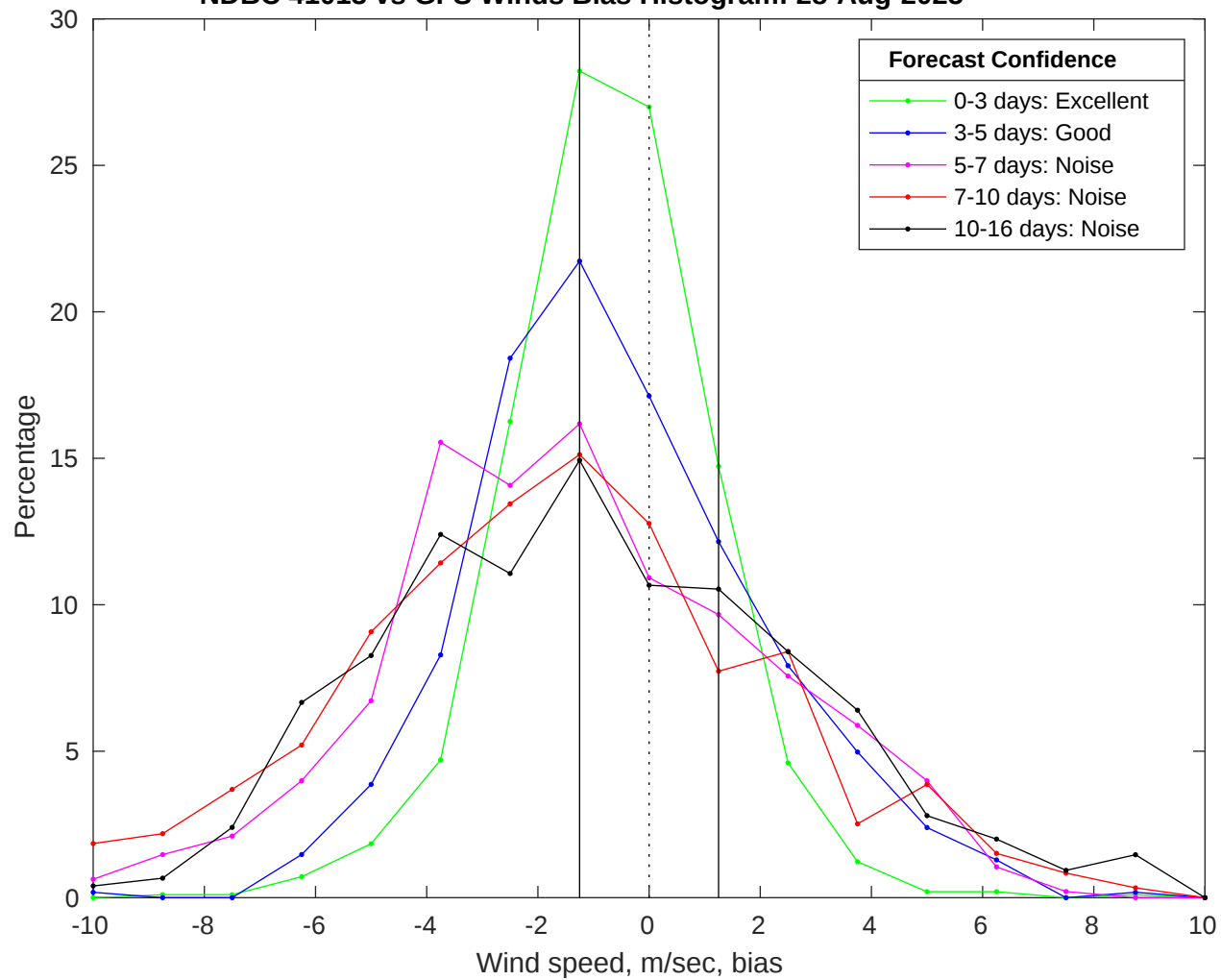
NDBC 41013 vs GFS Winds Bias Histogram: 28-Aug-2025
