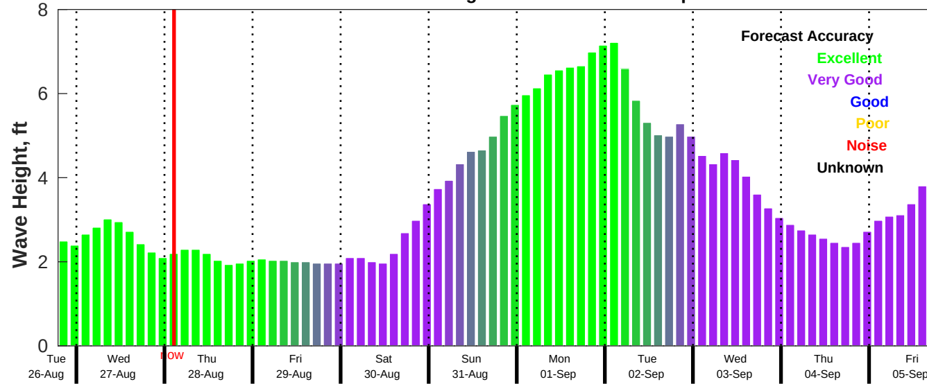
CMEMS Wave Forecast for NDBC 41013 from 26-Aug-2025 19:00:00 to 05-Sep-2025 19:00:00
