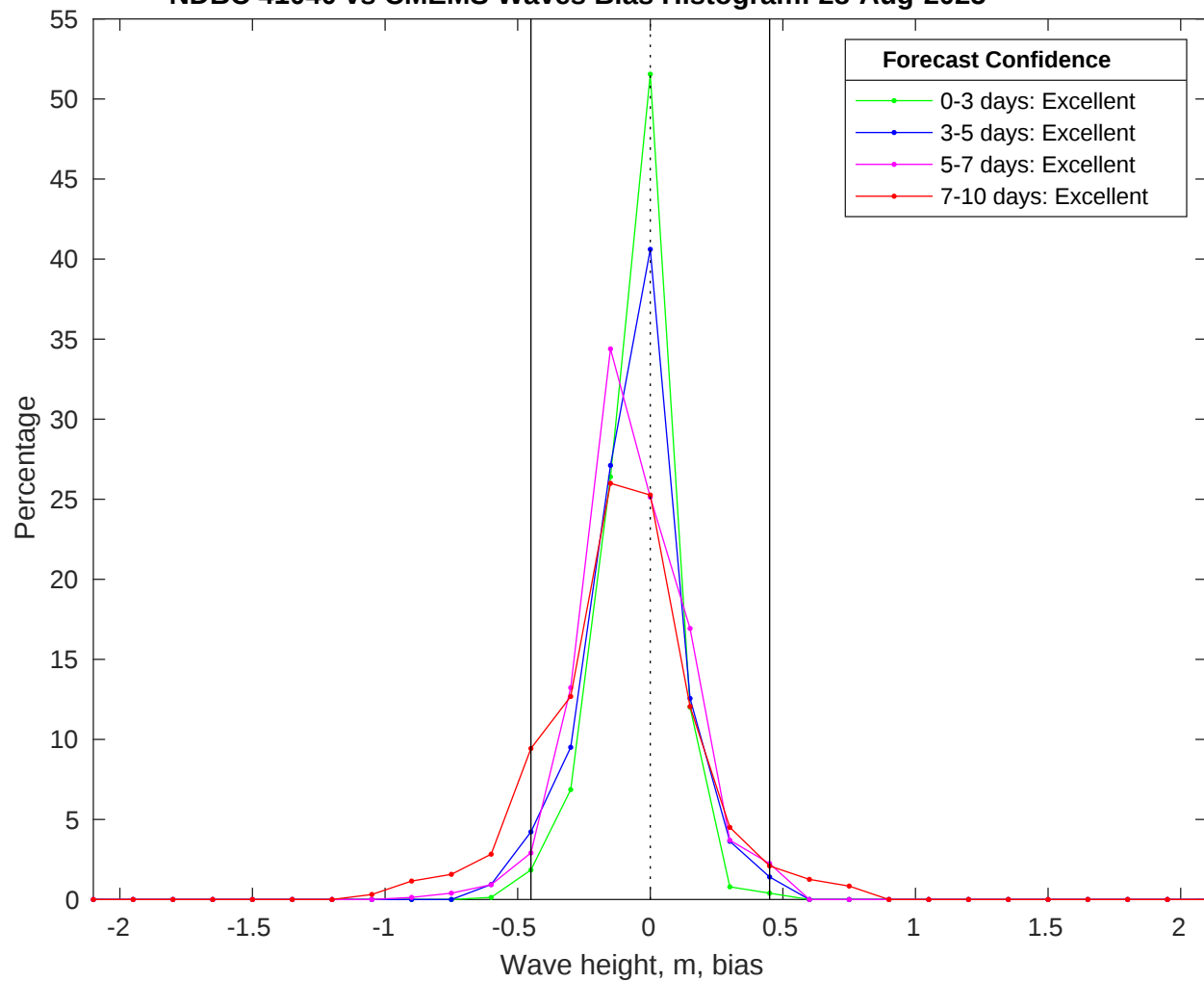
NDBC 41040 vs CMEMS Waves Bias Histogram: 28-Aug-2025
