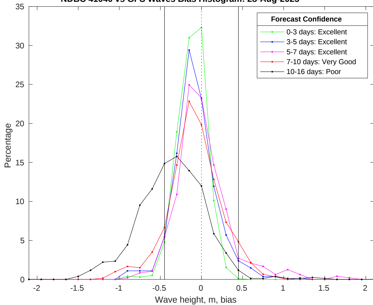
NDBC 41040 vs GFS Waves Bias Histogram: 28-Aug-2025
