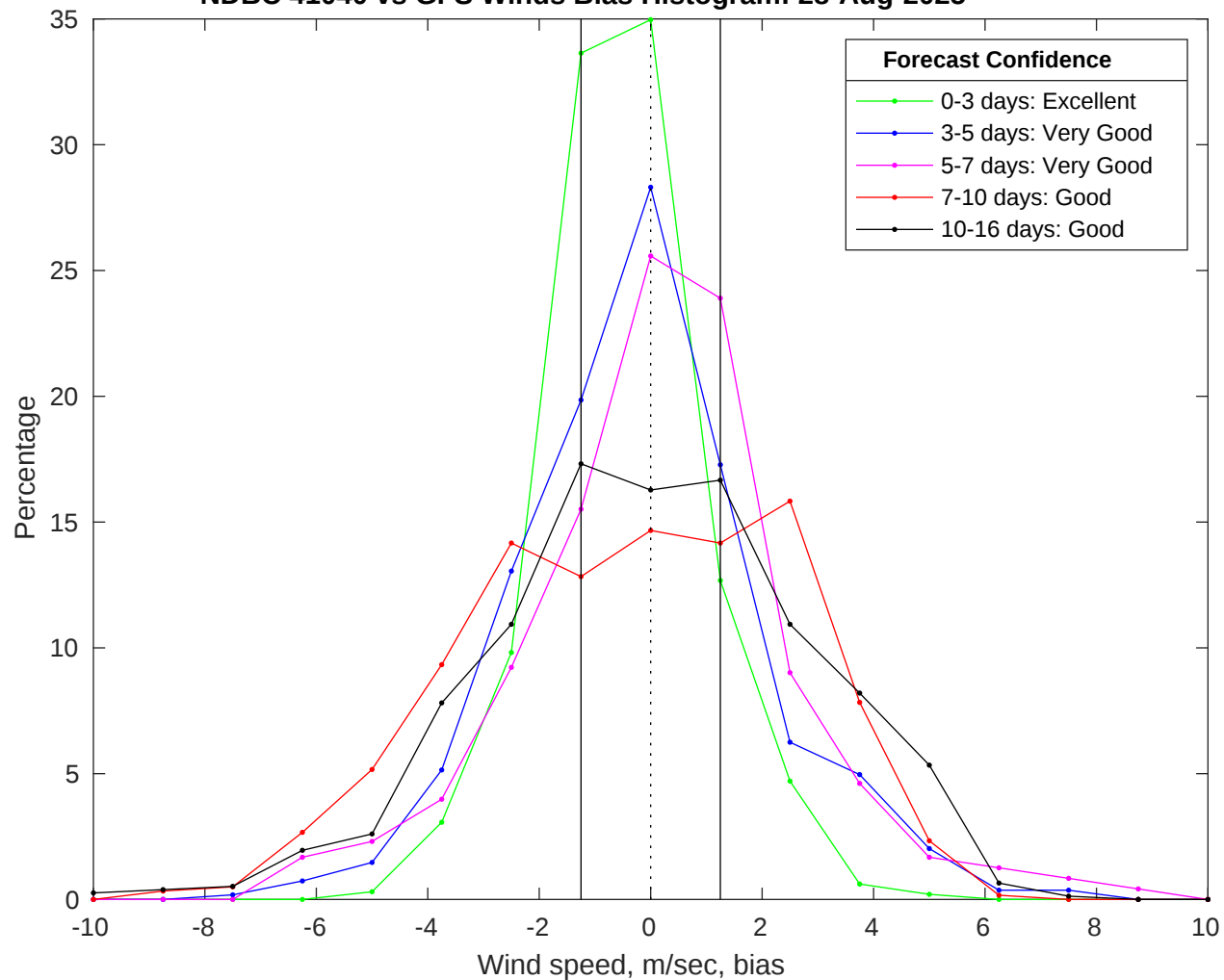
NDBC 41040 vs GFS Winds Bias Histogram: 28-Aug-2025
