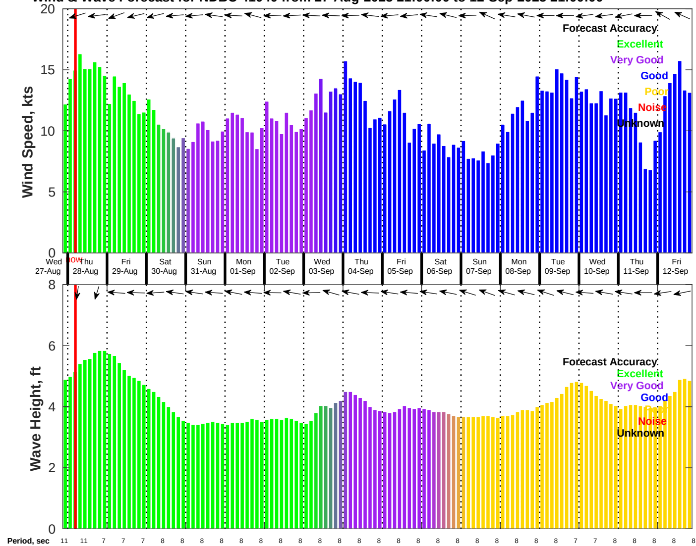
Wind & Wave Forecast for NDBC 41040 from 27-Aug-2025 21:00:00 to 12-Sep-2025 21:00:00
