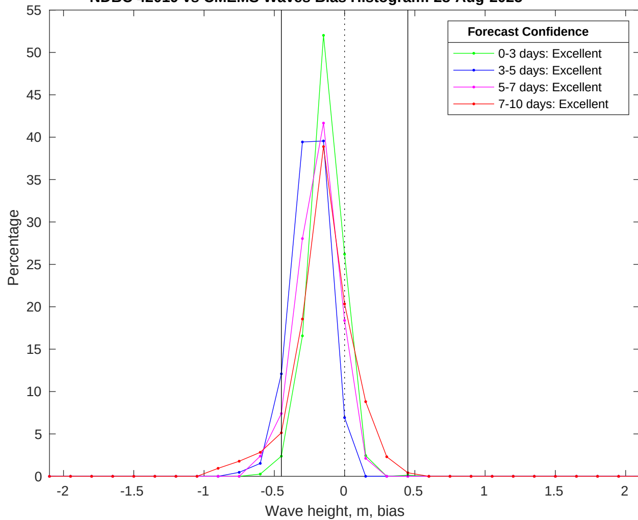
NDBC 42019 vs CMEMS Waves Bias Histogram: 28-Aug-2025
