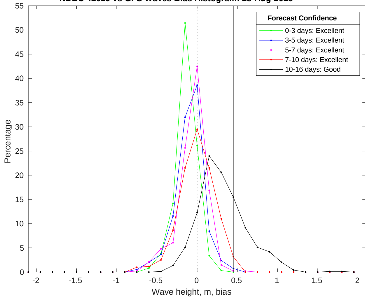
NDBC 42019 vs GFS Waves Bias Histogram: 28-Aug-2025
