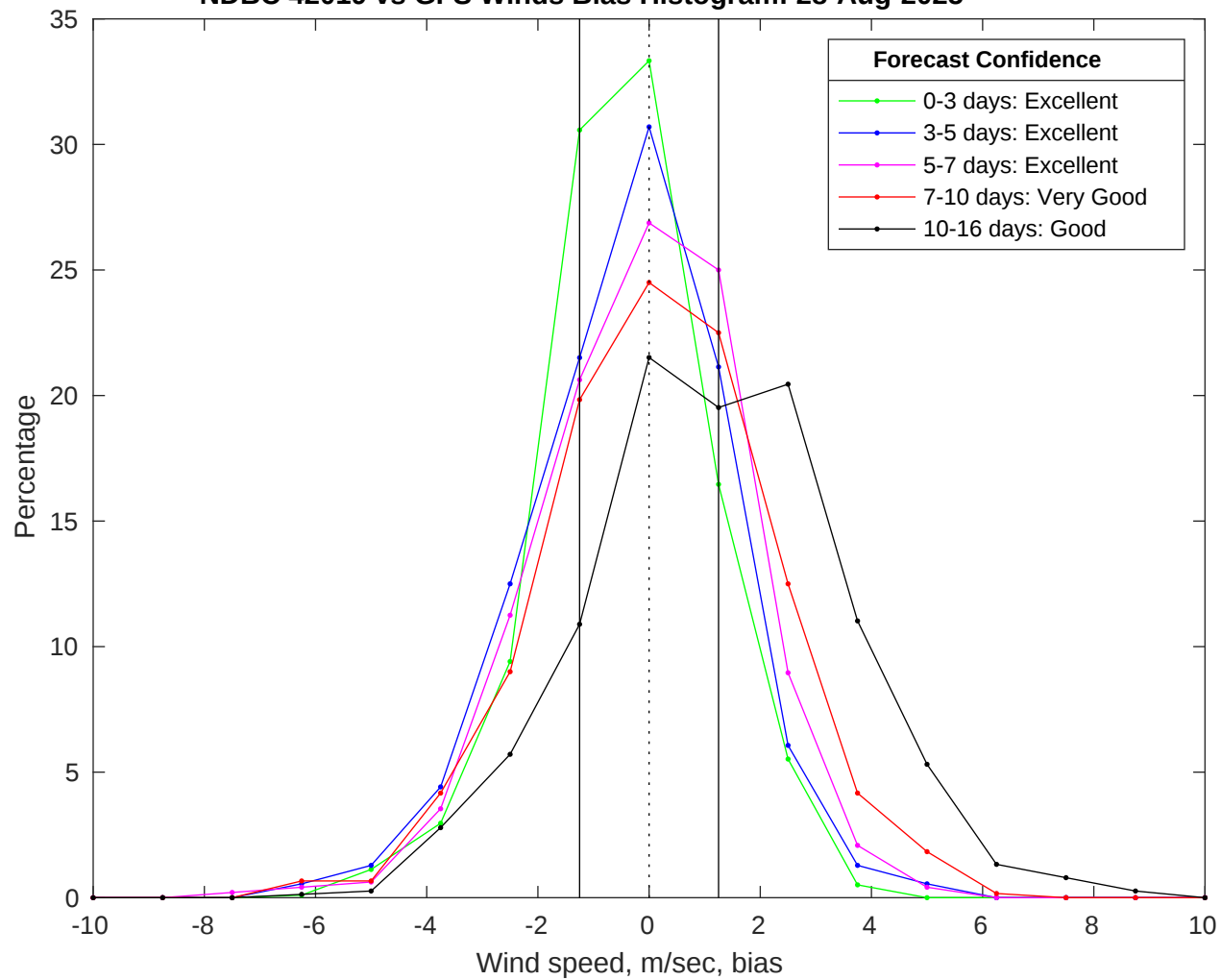
NDBC 42019 vs GFS Winds Bias Histogram: 28-Aug-2025
