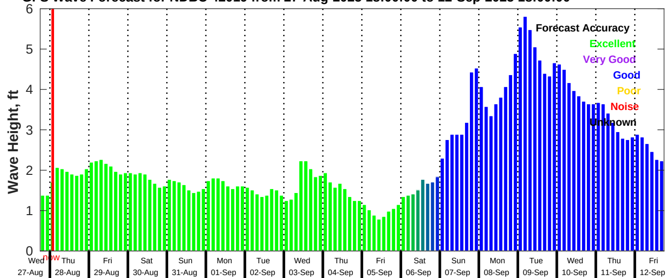
GFS Wave Forecast for NDBC 42019 from 27-Aug-2025 18:00:00 to 12-Sep-2025 18:00:00
