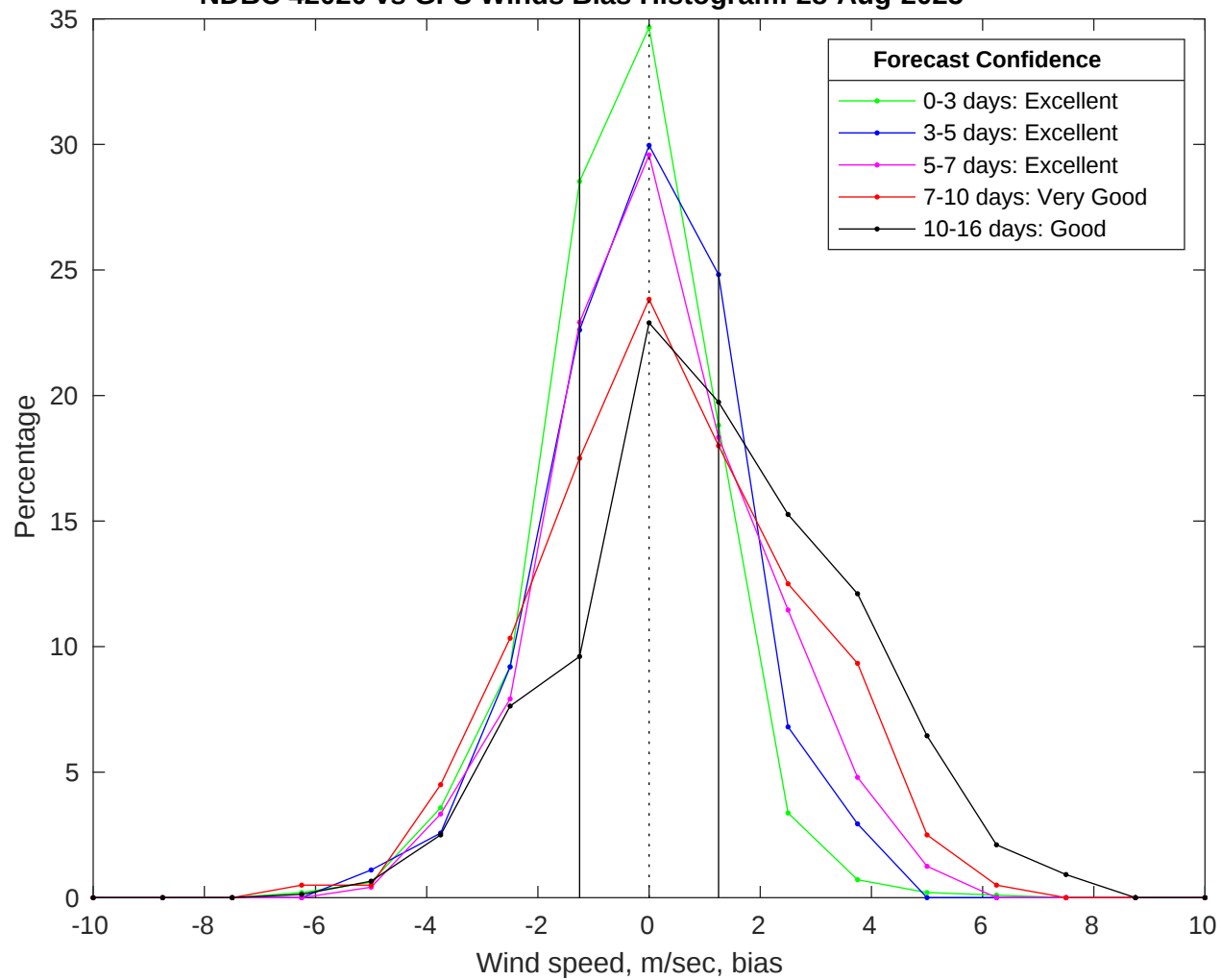
NDBC 42020 vs GFS Winds Bias Histogram: 28-Aug-2025
