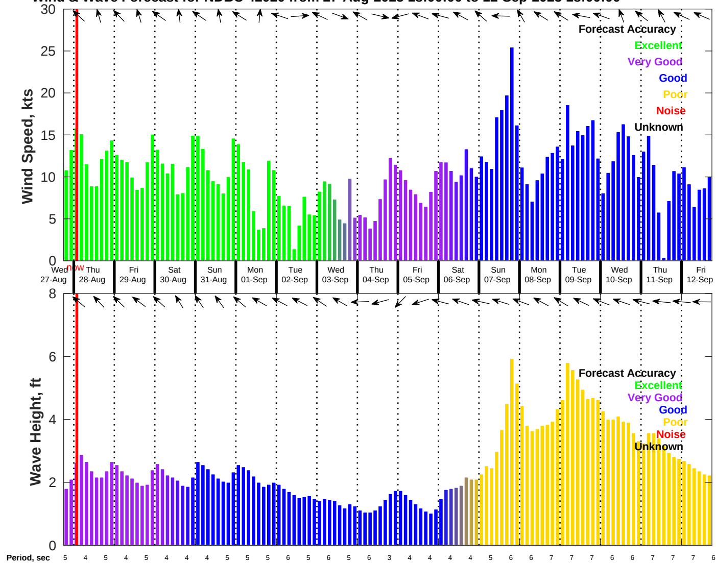
Wind & Wave Forecast for NDBC 42020 from 27-Aug-2025 18:00:00 to 12-Sep-2025 18:00:00
