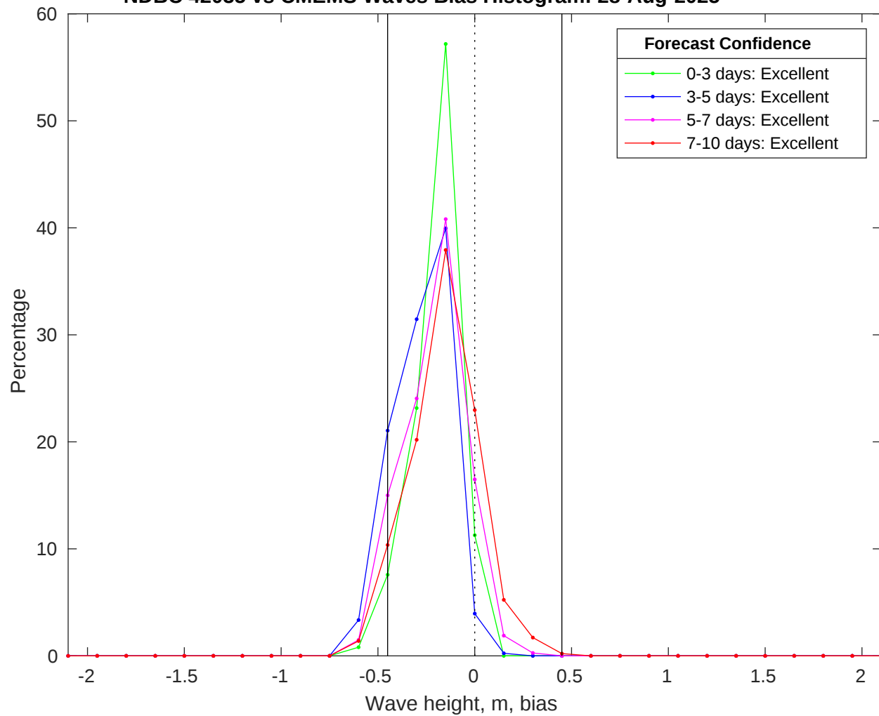
NDBC 42035 vs CMEMS Waves Bias Histogram: 28-Aug-2025
