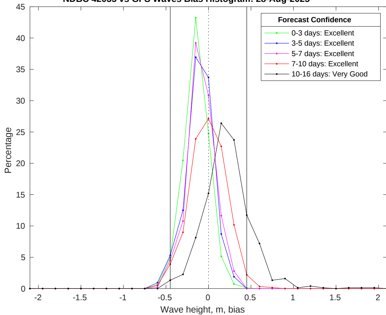
NDBC 42035 vs GFS Waves Bias Histogram: 28-Aug-2025
