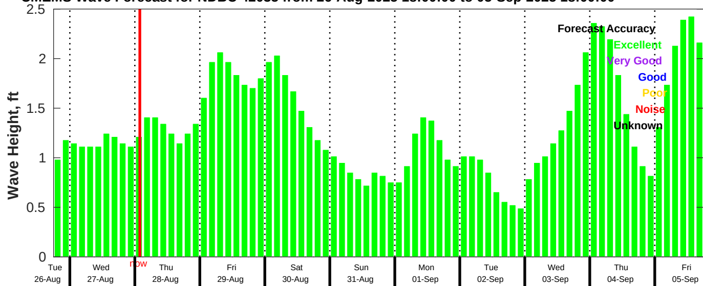
CMEMS Wave Forecast for NDBC 42035 from 26-Aug-2025 18:00:00 to 05-Sep-2025 18:00:00
