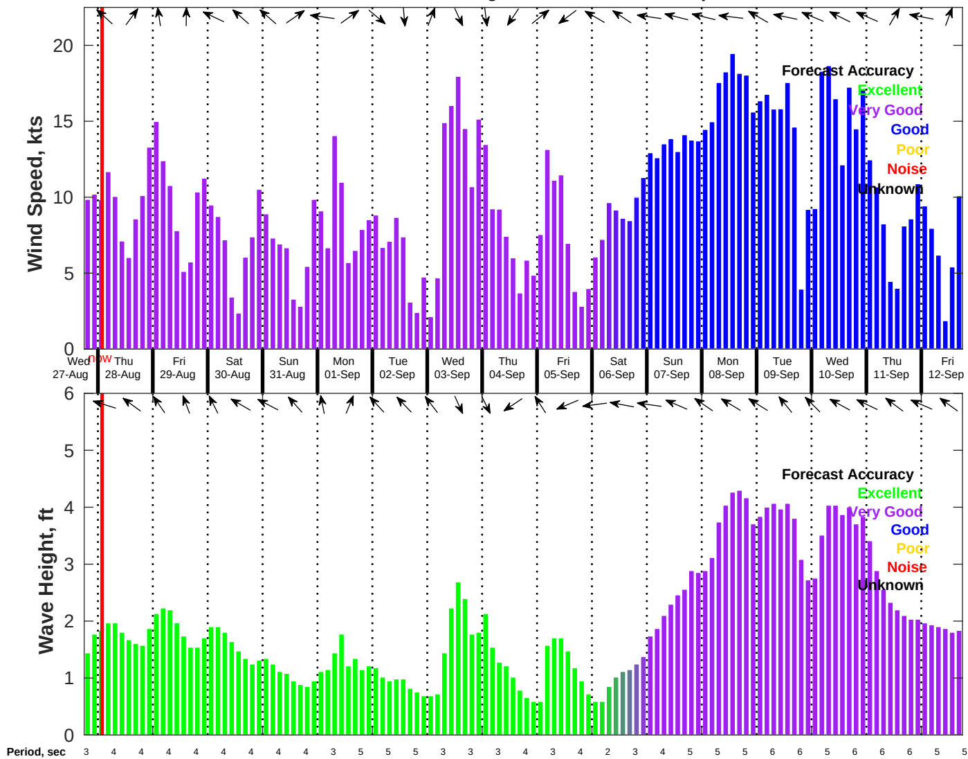
Wind & Wave Forecast for NDBC 42035 from 27-Aug-2025 18:00:00 to 12-Sep-2025 18:00:00
