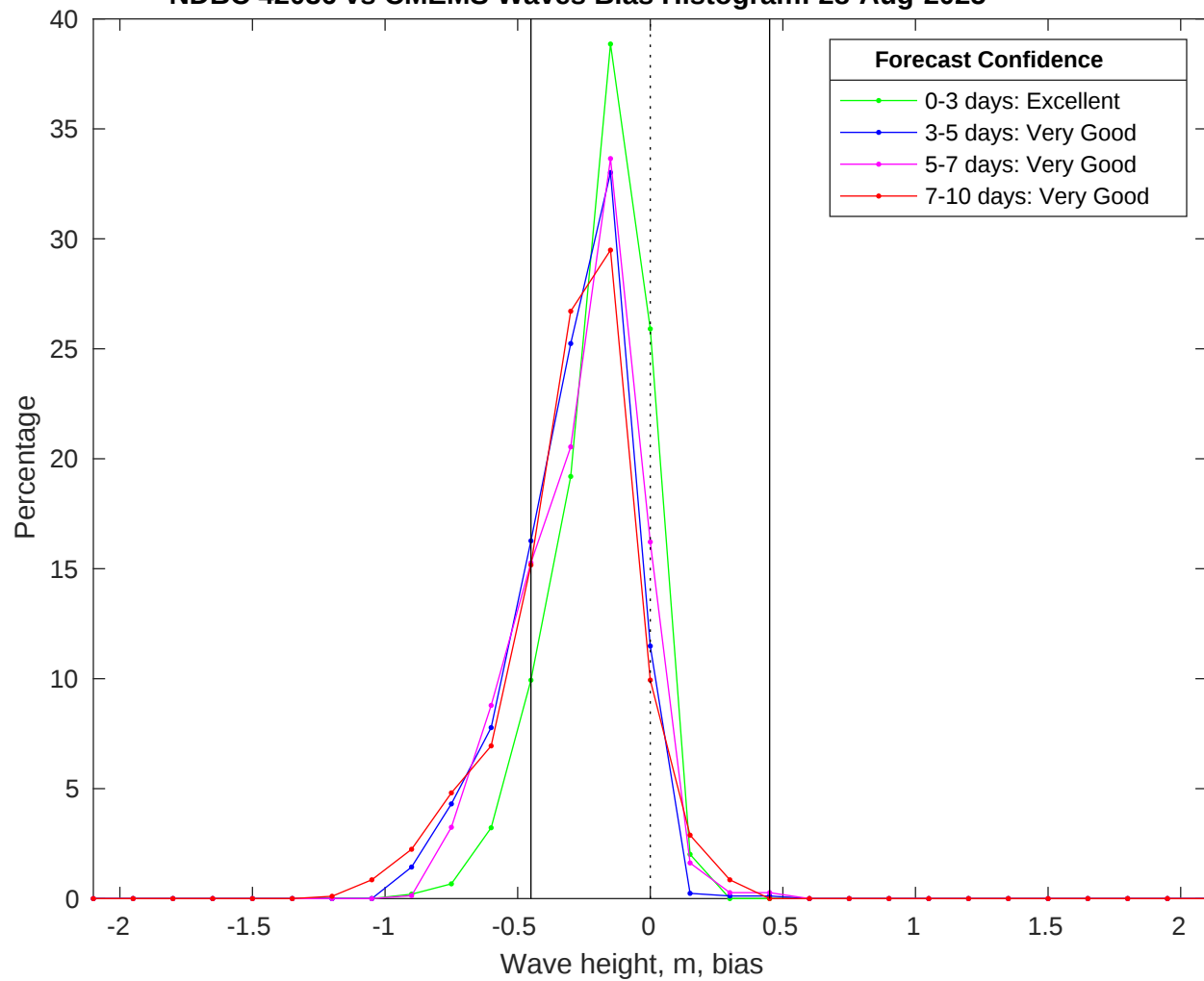
NDBC 42036 vs CMEMS Waves Bias Histogram: 28-Aug-2025
