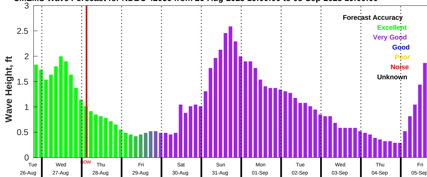
CMEMS Wave Forecast for NDBC 42036 from 26-Aug-2025 19:00:00 to 05-Sep-2025 19:00:00
