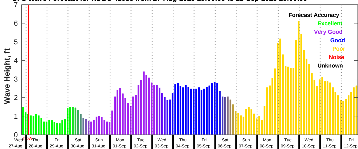
GFS Wave Forecast for NDBC 42036 from 27-Aug-2025 19:00:00 to 12-Sep-2025 19:00:00
