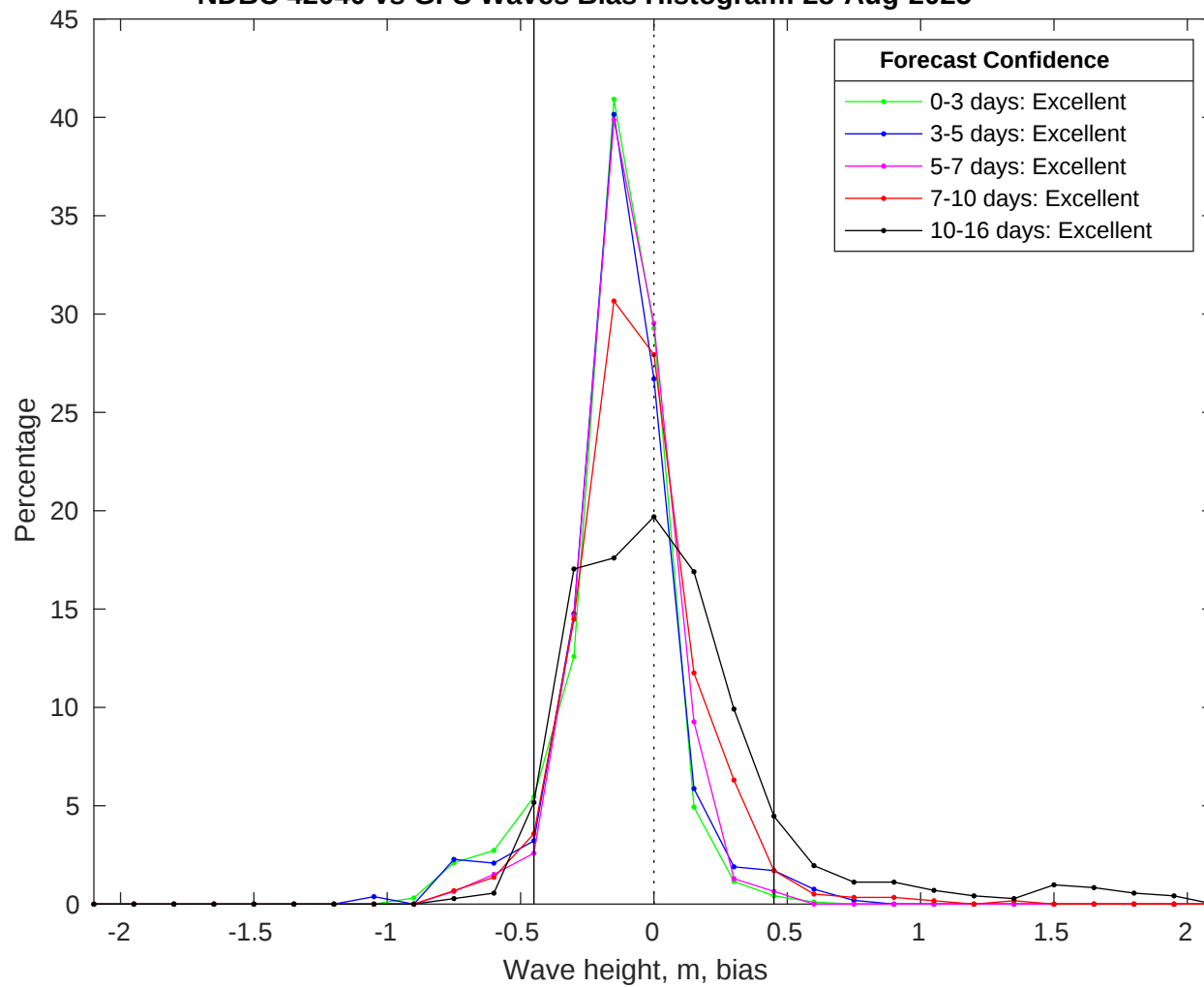
NDBC 42040 vs GFS Waves Bias Histogram: 28-Aug-2025
