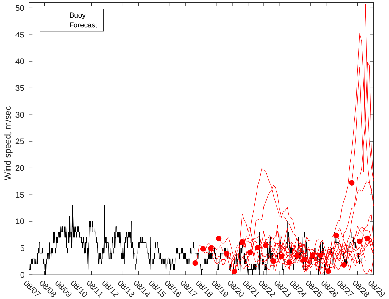
NDBC 42040 vs GFS Winds: 10 to 16 day forecast
