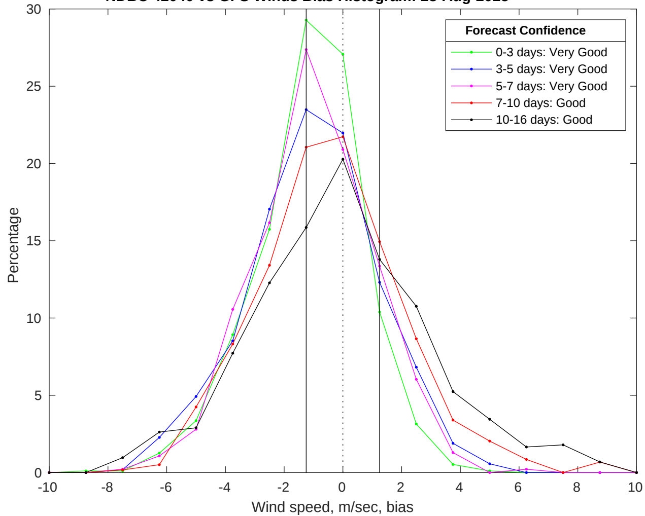
NDBC 42040 vs GFS Winds Bias Histogram: 28-Aug-2025
