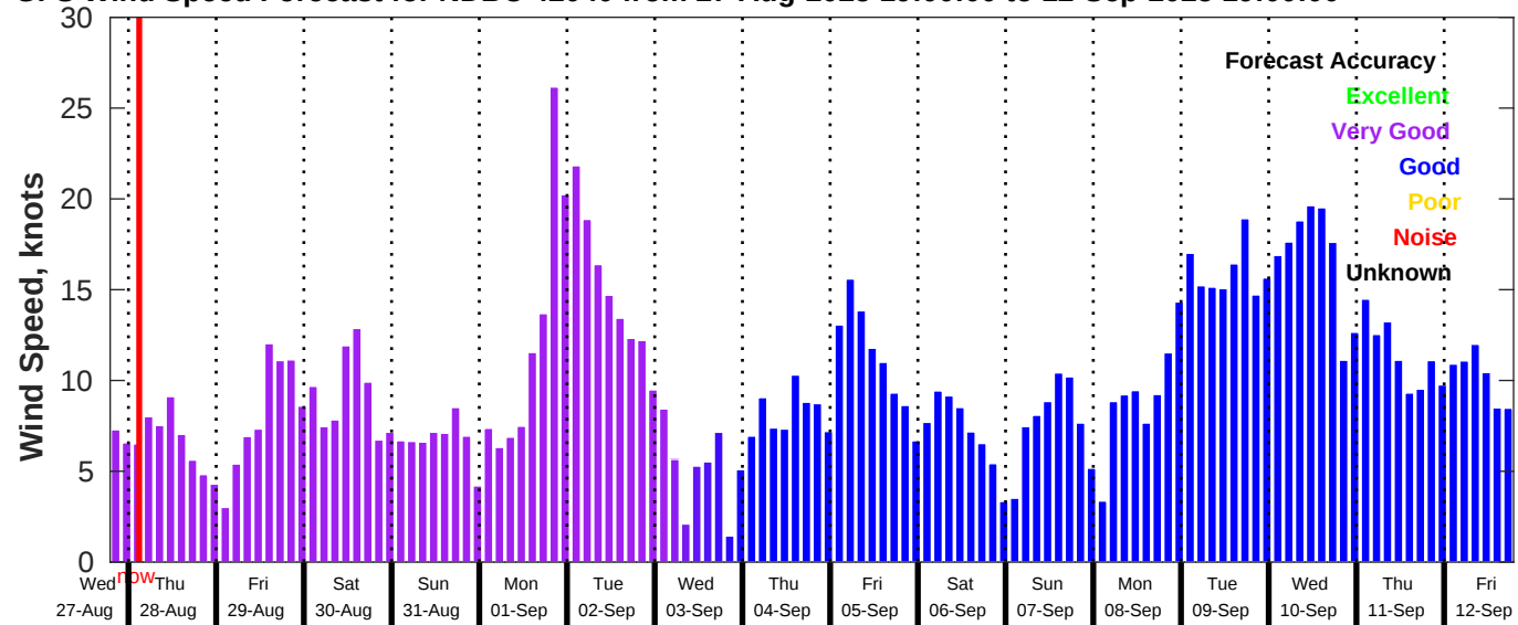
GFS Wind Speed Forecast for NDBC 42040 from 27-Aug-2025 19:00:00 to 12-Sep-2025 19:00:00
