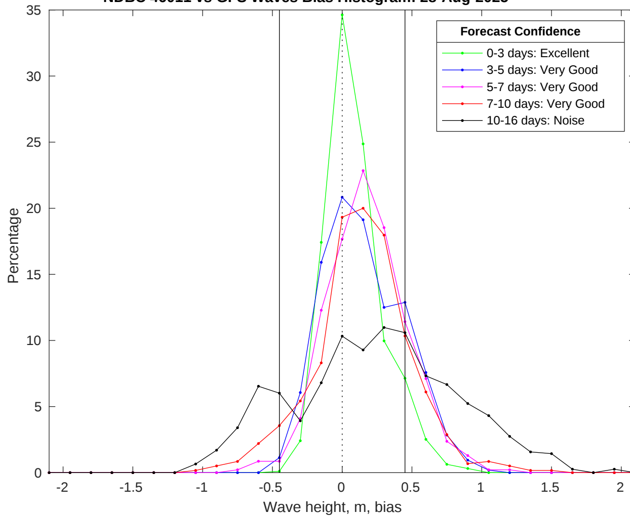
NDBC 46011 vs GFS Waves Bias Histogram: 28-Aug-2025
