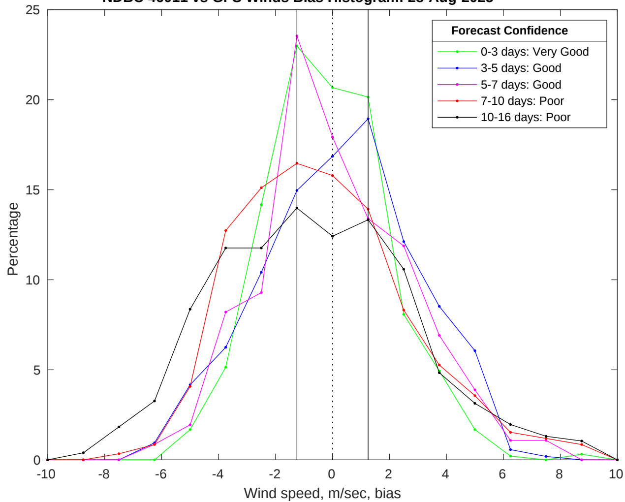
NDBC 46011 vs GFS Winds Bias Histogram: 28-Aug-2025
