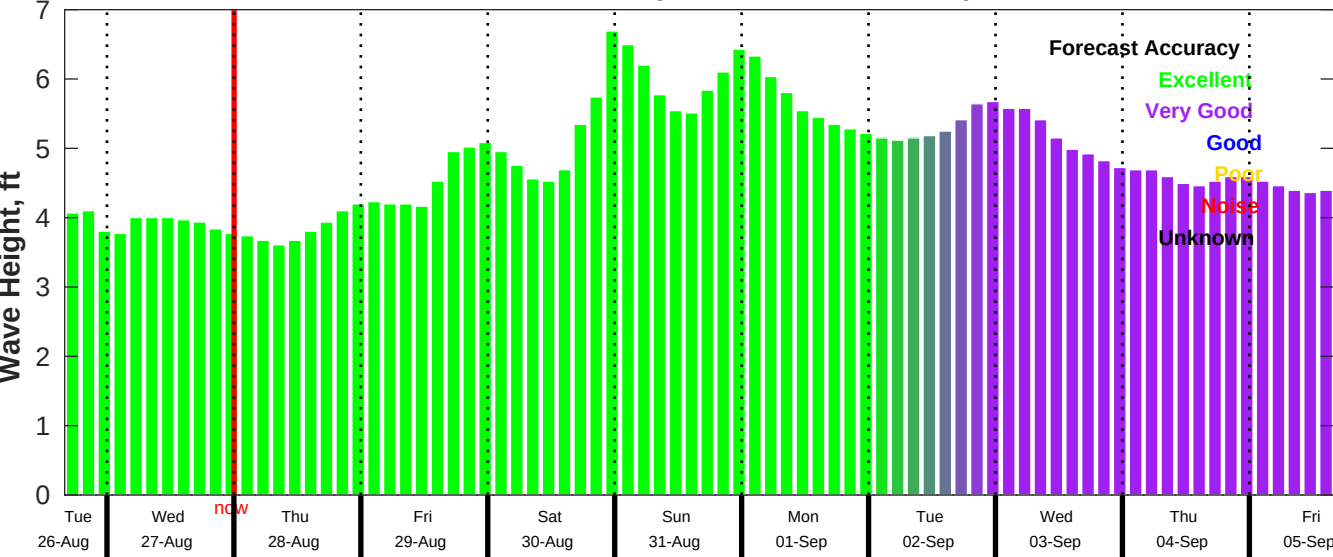
CMEMS Wave Forecast for NDBC 46011 from 26-Aug-2025 16:00:00 to 05-Sep-2025 16:00:00
