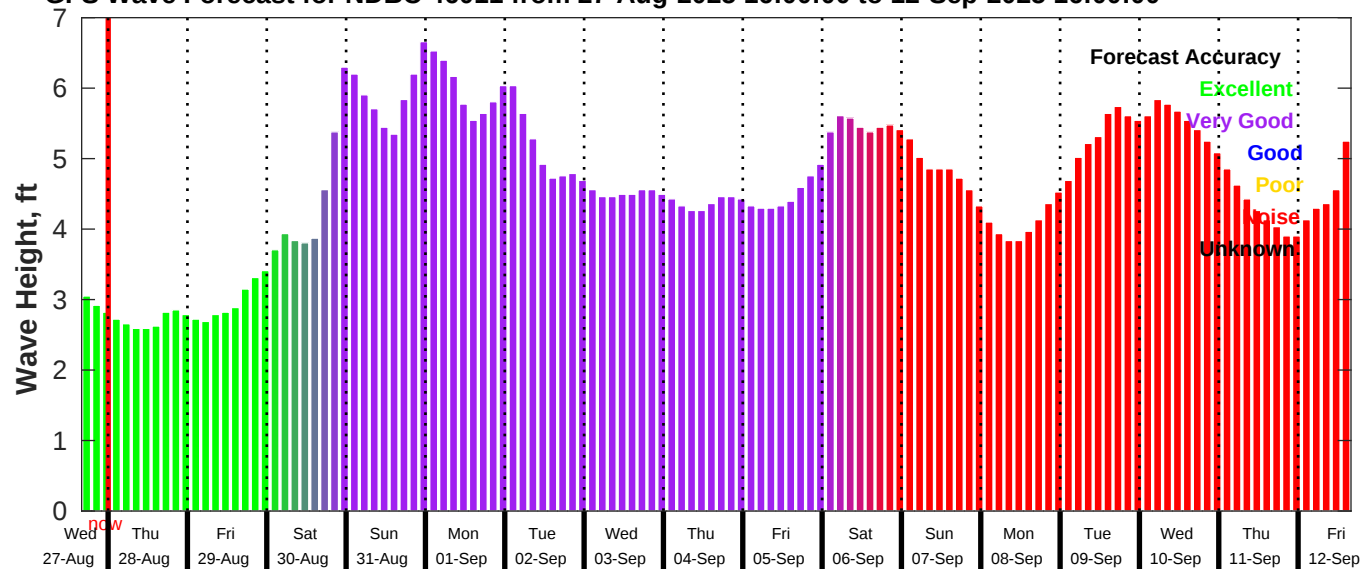
GFS Wave Forecast for NDBC 46011 from 27-Aug-2025 16:00:00 to 12-Sep-2025 16:00:00
