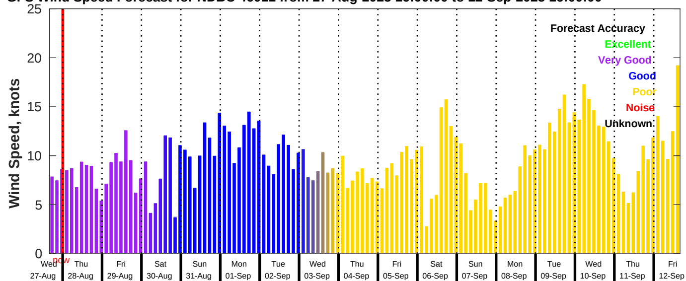
GFS Wind Speed Forecast for NDBC 46011 from 27-Aug-2025 16:00:00 to 12-Sep-2025 16:00:00
